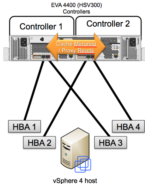
Figure 4. EVA/vSphere 4.x and 5.x direct-connect topology
