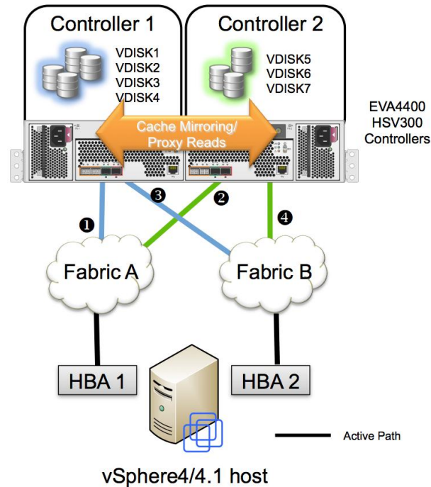
Figure 7. EVA connectivity with vSphere 4.x/5.x
