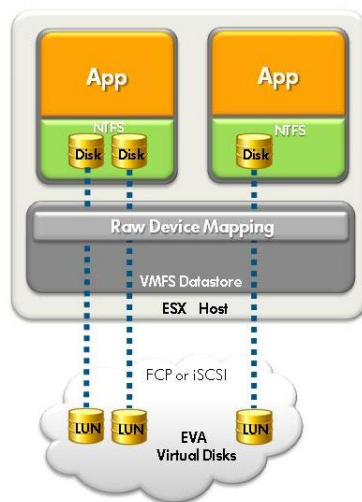
Figure 12. RDM datastore
