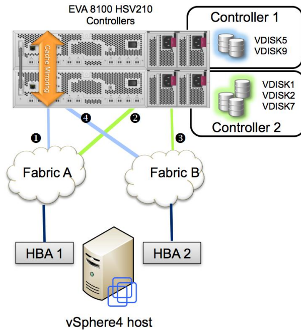
Figure C-1. Sample vSphere 4.x/5.x environment featuring an HP 8100 Enterprise Virtual Array with two four-port HSV210 controllers
