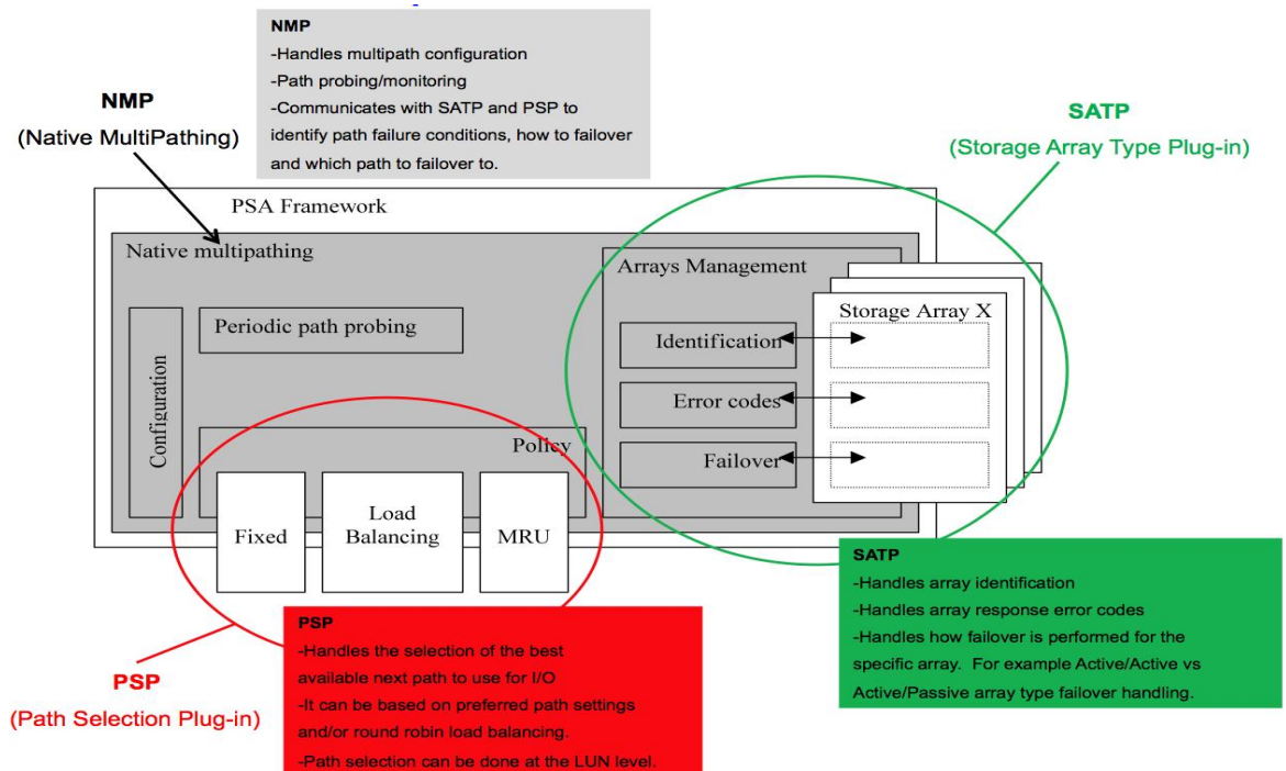
Figure 9. vSphere 4.x and 5.x multi-pathing stack
